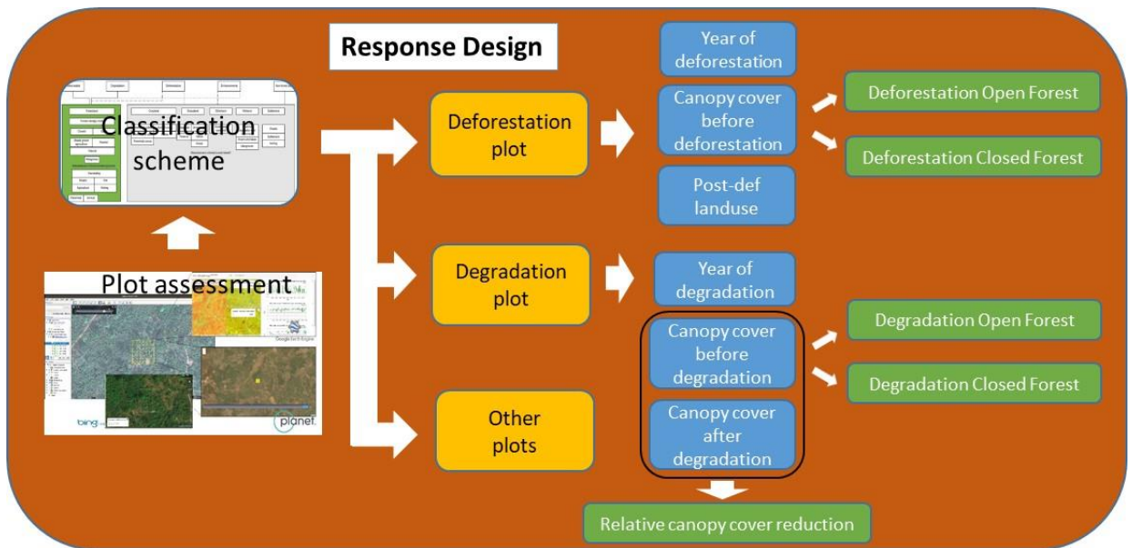
Figure 28 Response Design
