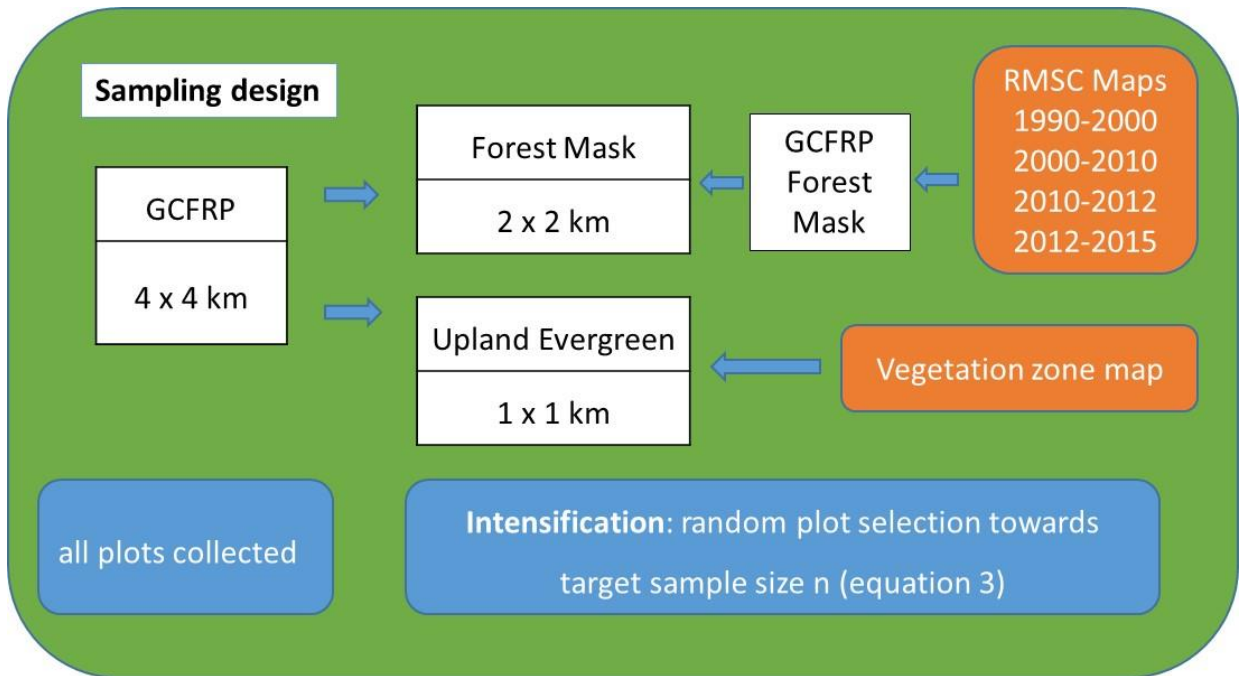
Figure 27 Sampling design
